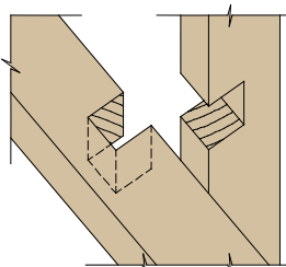
Half Lap
