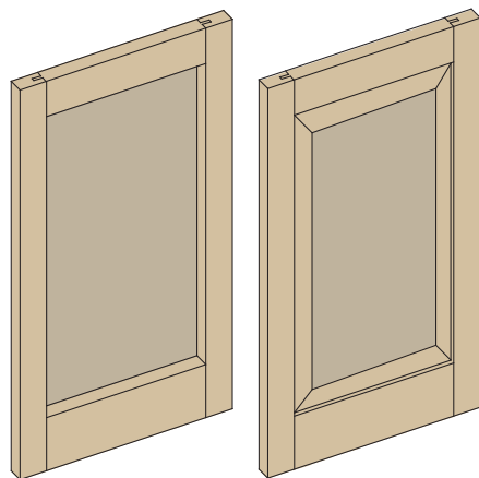
Flat Panel
