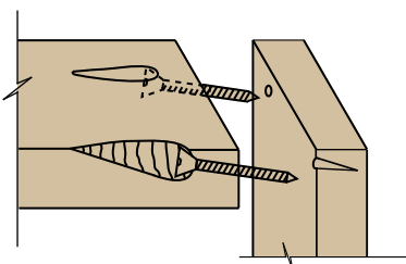
Pocket Screw
