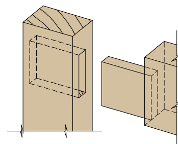
Through Mortise & Tenon
